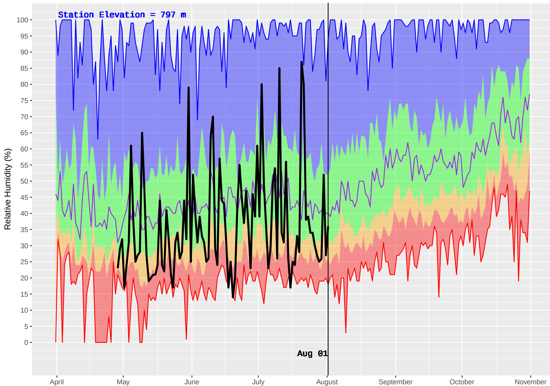
VALEMOUNT HUB (194) : Historical (1970–2016) and Current (2018) Daily Relative Humidity
