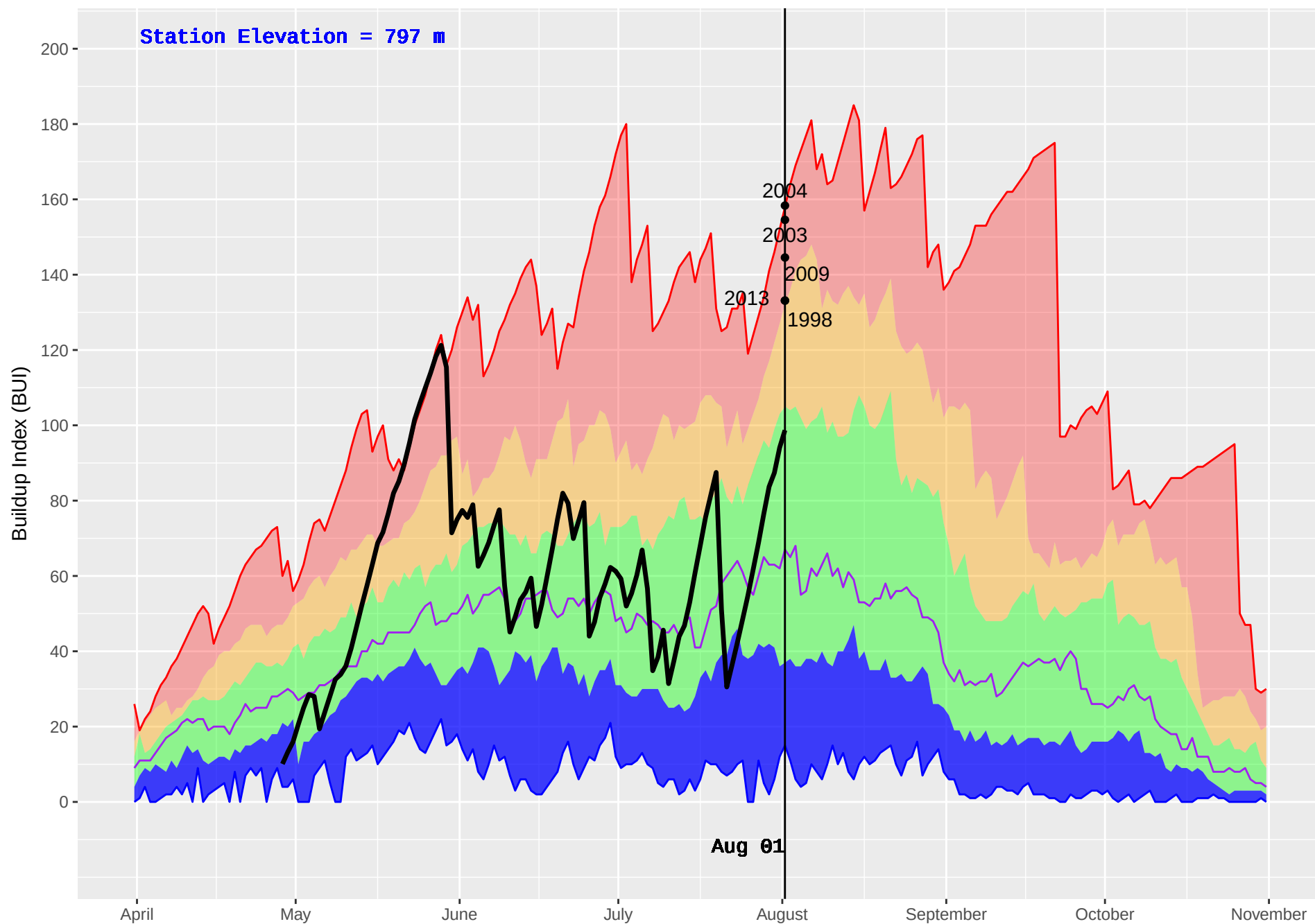
VALEMOUNT HUB (194) : Historical (1970–2016) and Current (2018) Daily Buildup Index (BUI)
